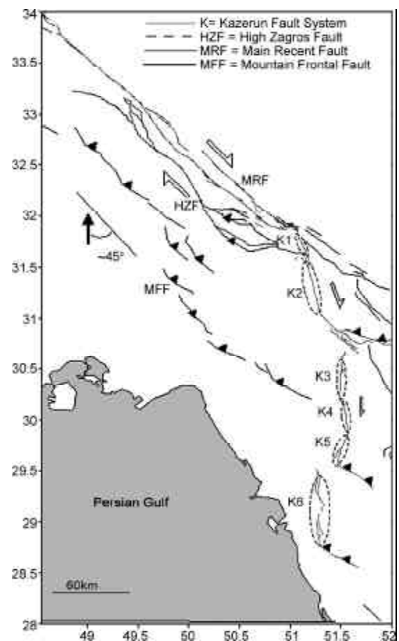
Figure 15. Fault segmentation of Kazerun Fault. The location is shown on Figure (1). Black-filled arrows show the convergence direction and the angle that it makes with the plate boundaries is shown. Open arrows demonstrate the strike-slip kinematics with southward decreasing in slip rate. Filled triangles show the thrust fault, see Figure (5) for location.
