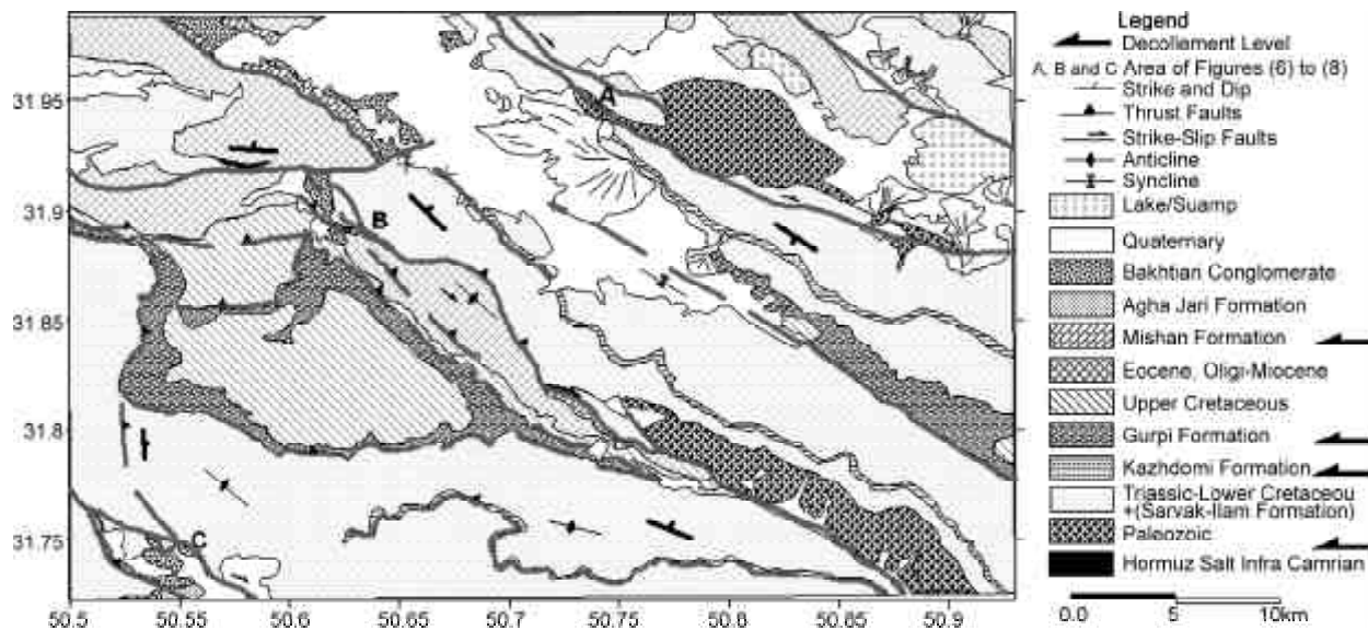
Figure 2. Geological and structural map of west-central High Zagros modified from Geological quadrangle map of Iran, Ardal sheet, sheet 6153, scale 1:100,000 [16]. The decollement horizons are indicated in legend by arrows. Intrusion of salts to the surface and manifestation along strike of the MRF and HZF reveal that the faults are probably originated beneath the basement. From seismic hazard point of view, the faults that cut the basement are more important and demonstrate the regional strain partitioning. A, B and C are located on the area of Figures (6) to (8).
