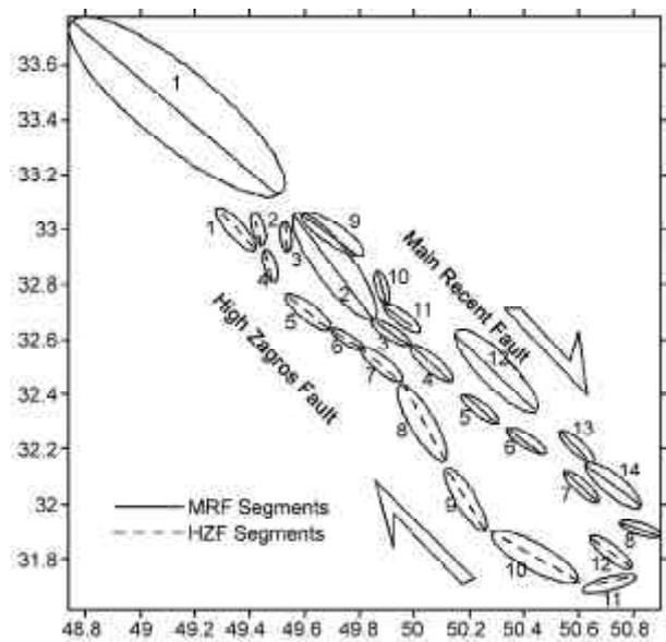
Figure 16. Fault segmentation along HZF and MRF using spot and Landsat satellite images and field work observations. The segments are separated by steps, see Figure (5) for location. The length of the segments is given in Table (1).
