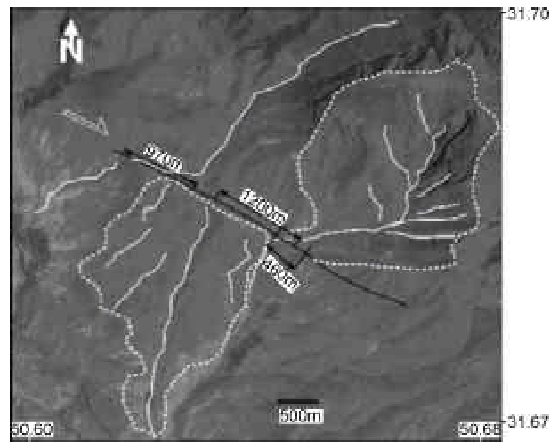
Figure 14. Alluvial fan on Landsat image displaced by HZF, see Figure (5) for location. Considering the age of 140ka, given by Authemayou et al [6] and at least 460m offset of fan, the slip rate and earthquake recurrence time were calculated, see Table (1). Notice the beheaded fan implying the presence of the compressional component along HZF.
